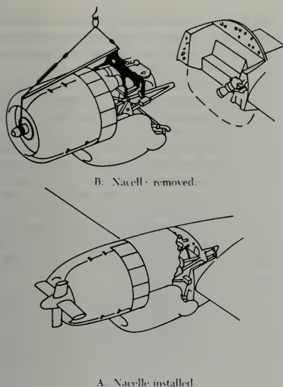
FIGURE 8-3. Separation line of a typical QECA.
